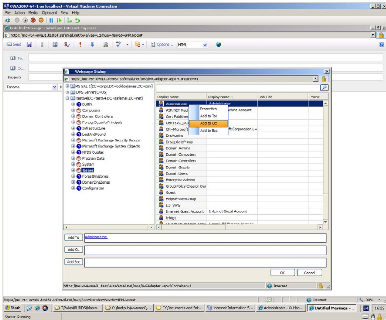
Figure 1. The MasterKeyPlus web client Address Book extension to Outlook Web Access 2007 user interface.
